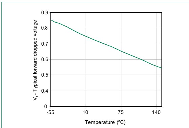
Figure 5: Forward Voltage
