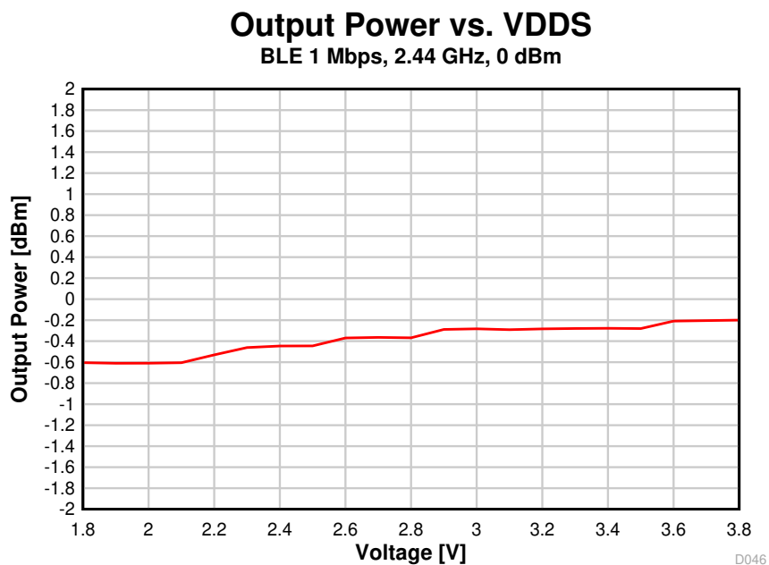
Figure 8-25. Output Power vs. Supply Voltage (VDDS) (BLE 1 Mbps, 2.44 GHz)
