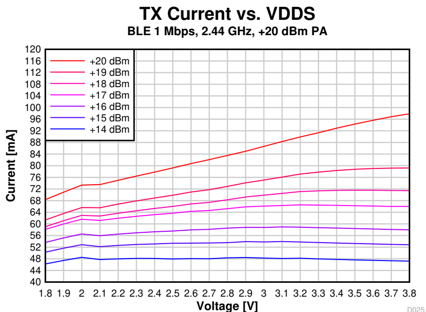
Figure 8-12. TX Current vs. Supply Voltage (VDDS) (BLE 1 Mbps, 2.44 GHz, +20 dBm PA)
