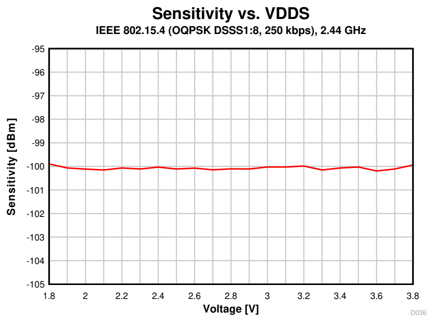
Figure 8-20. Sensitivity vs. Supply Voltage (VDD) (250 kbps, 2.44 GHz)
