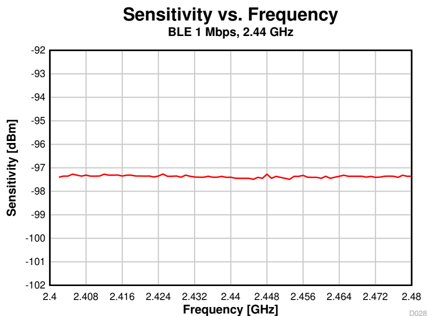
Figure 8-14. Sensitivity vs. Frequency (BLE 1 Mbps, 2.44 GHz)
