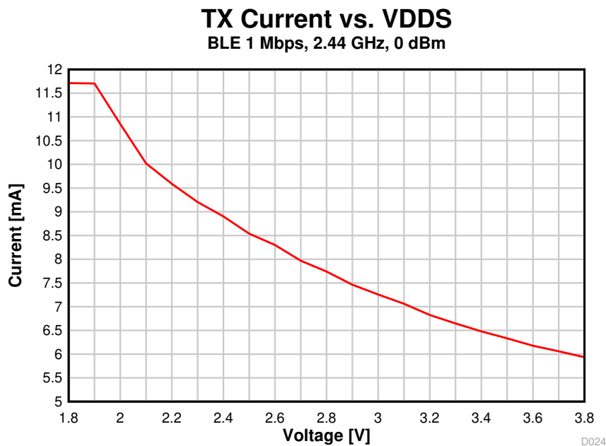
Figure 8-11. TX Current vs. Supply Voltage (VDD5) (BLE 1 Mbps, 2.44 GHz)
