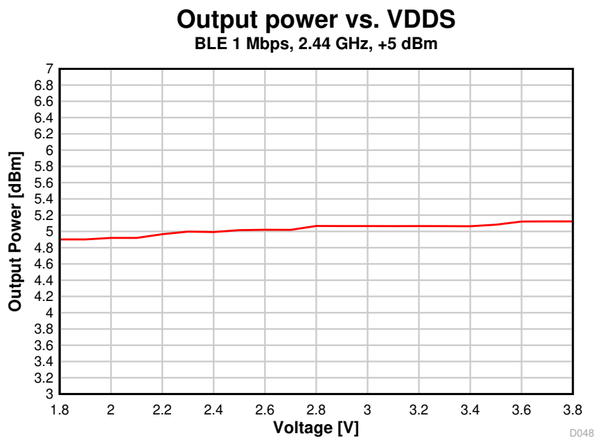
Figure 8-26. Output Power vs. Supply Voltage (VDDS) (BLE 1 Mbps, 2.44 GHz, +5 dBm)
