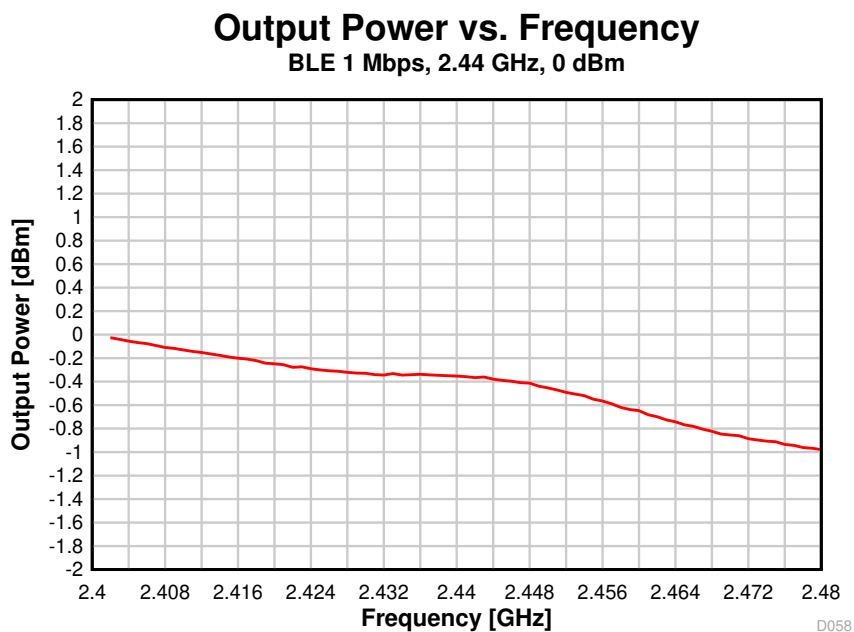
Figure 8-29. Output Power vs. Frequency (BLE 1 Mbps, 2.44 GHz)
