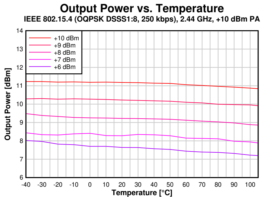
Figure 8-24. Output Power vs. Temperature (2.44 GHz, +10 dBm PA)
