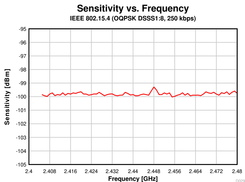
Figure 8-15. Sensitivity vs. Frequency (250 kbps, 2.44 GHz)
