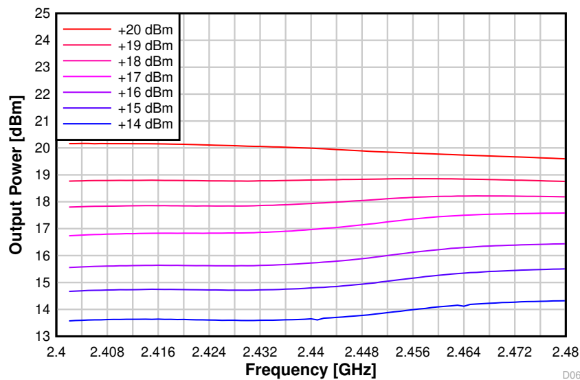
Figure 8-56. Output Power vs. Frequency (BLE 1 Mbps, 2.44 GHz, +20 dBm PA)
