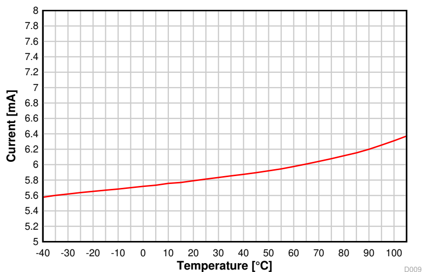
Figure 8-8. RX Current vs. Temperature (50 kbps, 868.3 MHz, VDDSD = 3.6 V)
